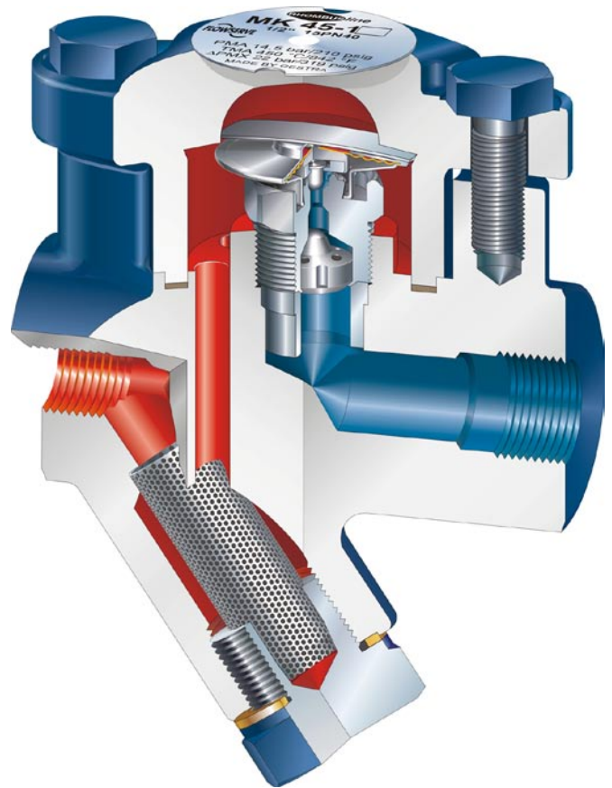
GESTRA Steam Trap RHOMBUSlineType MK 45
